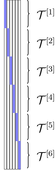
Figure 2.4 \rho = 1 and \beta = 1 case
