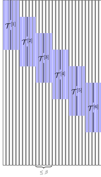
Figure 2.3 \rho = 3 and \beta = 5 case
