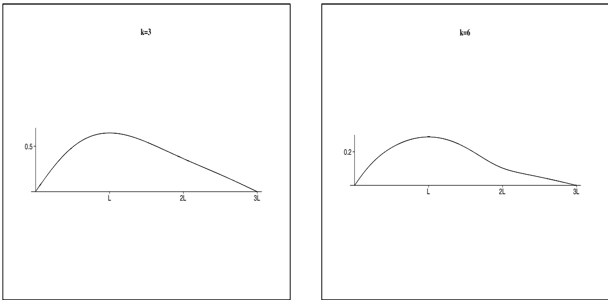
FIGURE 11. Hitchin metrics on [0, 3L] .
