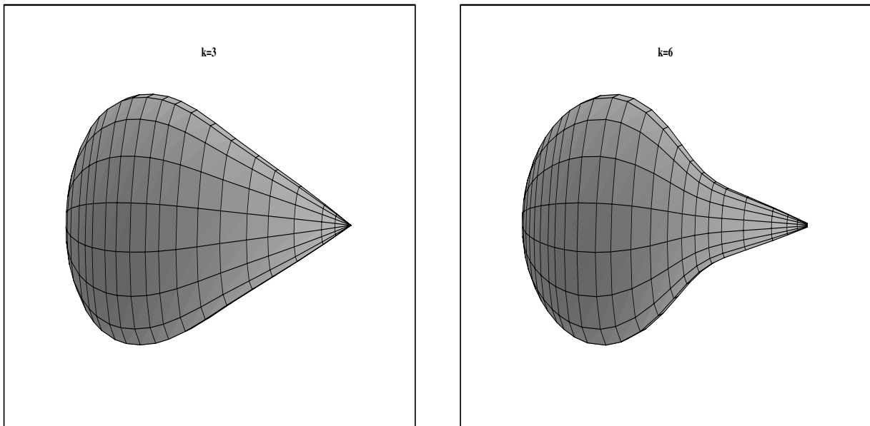
FIGURE 12. Fixed point orbifold 2-spheres in Hitchin metrics.
